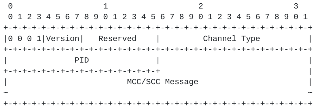
Figure 1: G-ACh MCC/SCC Packet
