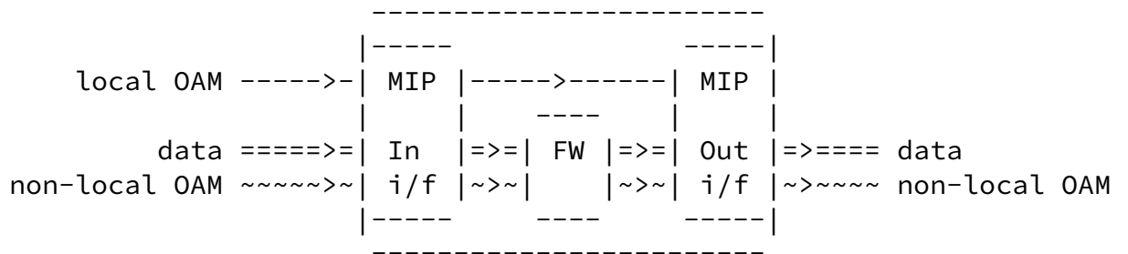
Figure 7: OAM Control Message Delivery Bypassing the Forwarding Engine
