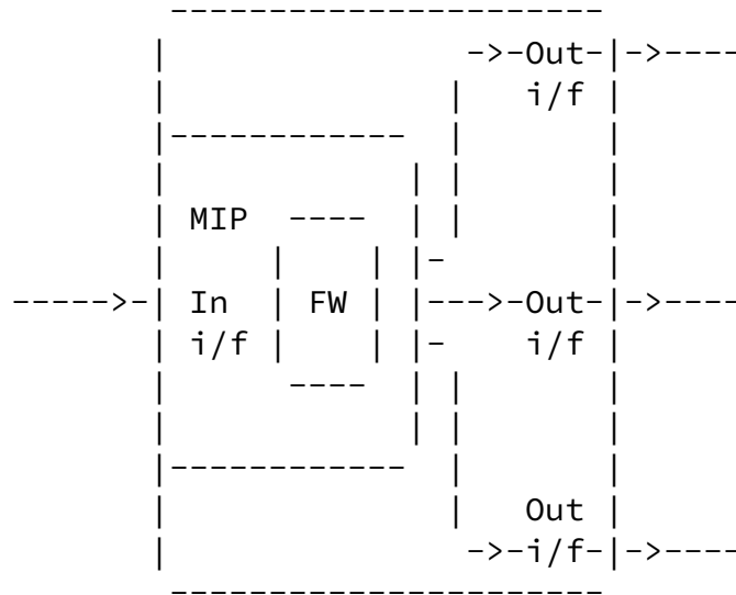
Figure 6: Abstract Functional Representation of Some Existing MPLS-TP Nodes Supporting P2MP
