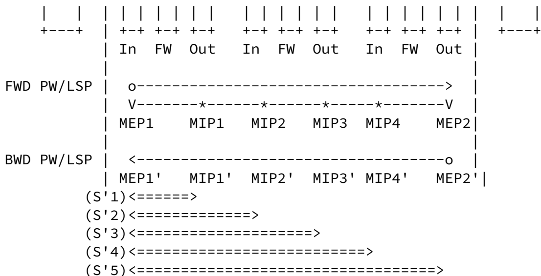
Figure 3: Example of OAM relying on per-interface MIPs and MEPs
