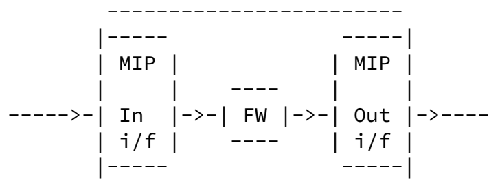
Figure 1: Abstract Functional Representation of an MPLS-TP Node
