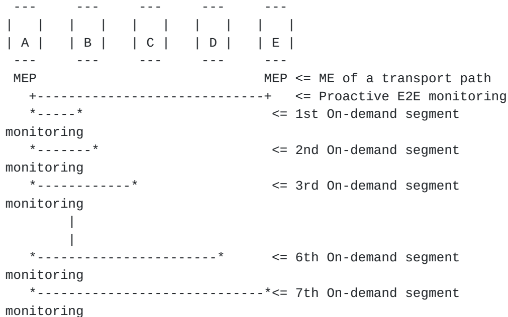
Figure 4 : One possible procedure to localize a fault point by sequential on-demand segment monitoring
