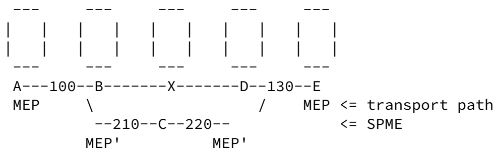
Figure 1 : An Example of a SPME setting
