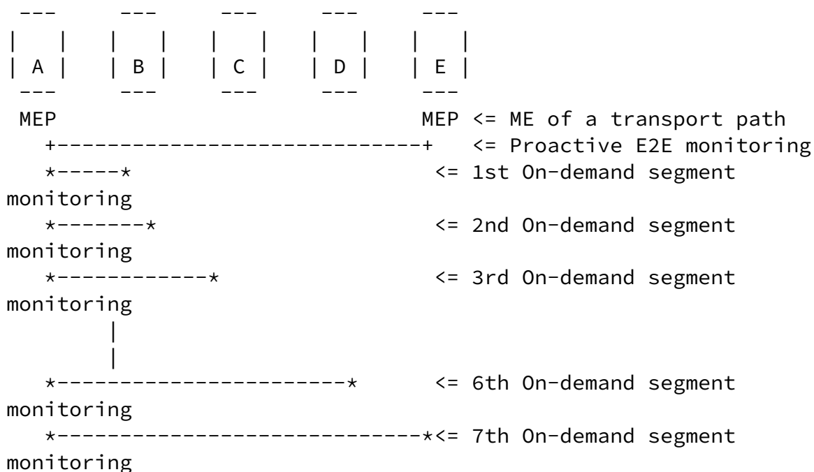
Figure 4 : One possible procedure to localize a fault point by sequential on-demand segment monitoring
