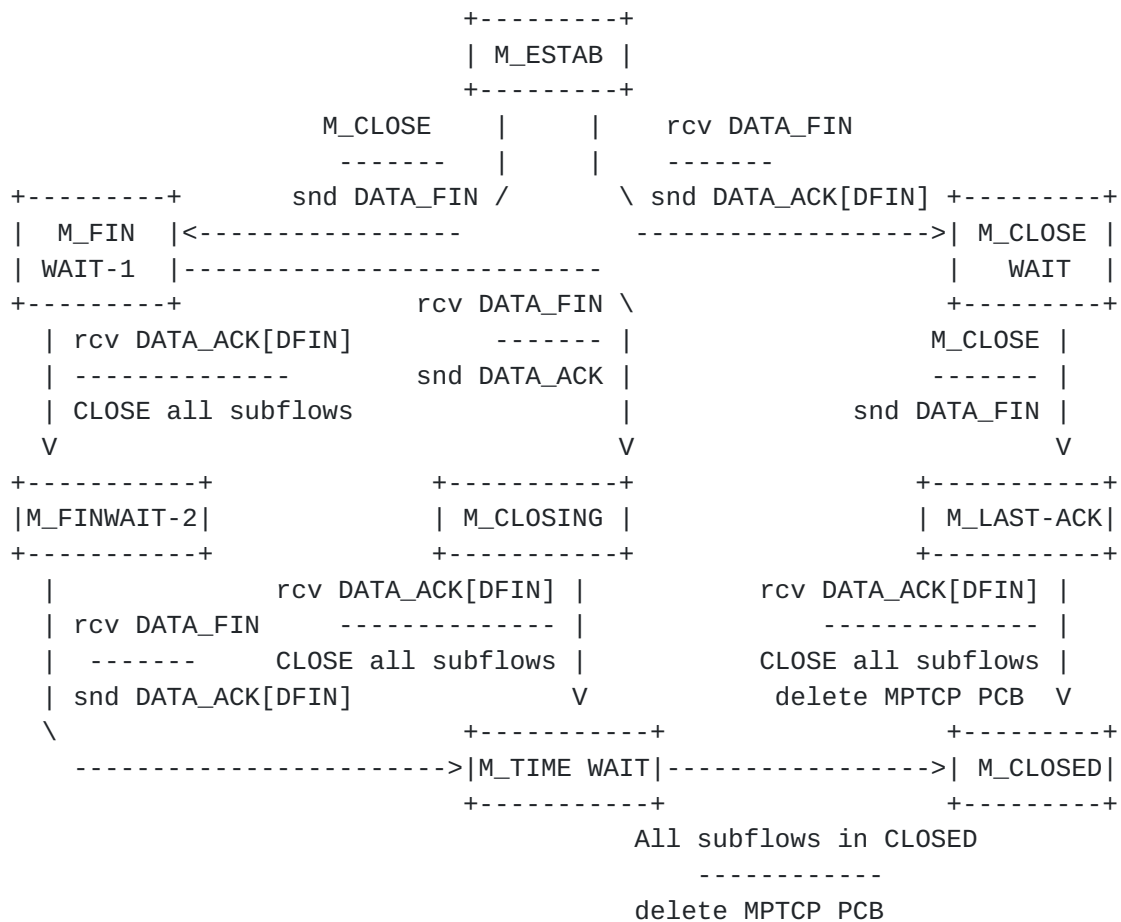
Figure 18: Finite State Machine for Connection Closure
