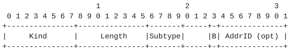
Figure 11: Change Subflow Priority (MP_PRI0) Option
