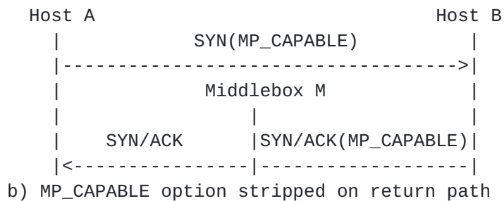
Figure 22: Connection Setup with Middleboxes that Strip Options from Packets
