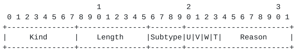
Figure 15: TCP RST Reason (MP_TCPRST) Option
