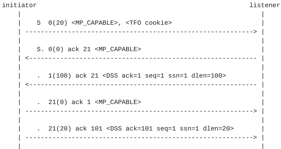
Figure 19: The listener supports TF0
