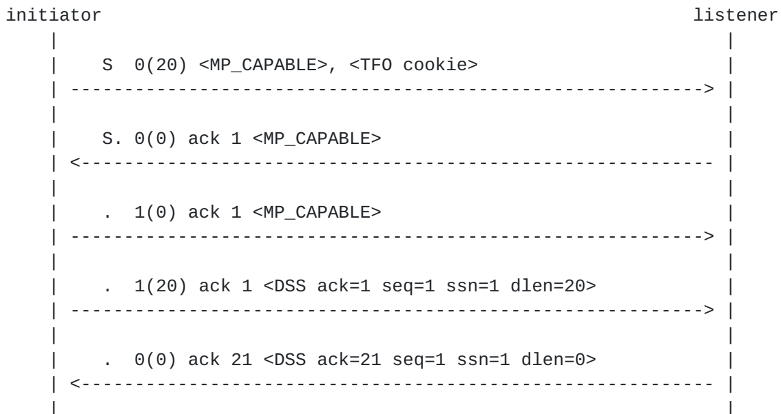
Figure 20: The listener does not support TF0
