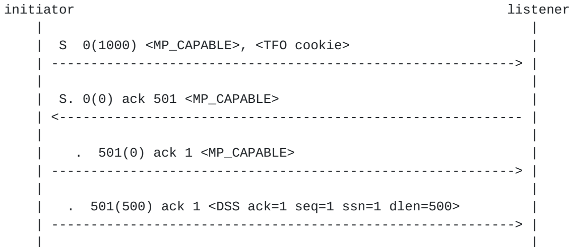
Figure 21: Partial data acknowledgement
