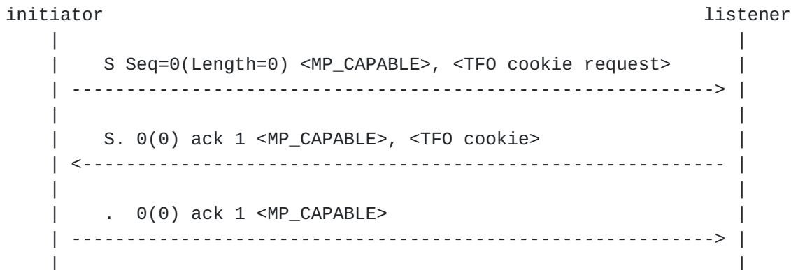
Figure 18: Cookie request - sequence number and length are annotated as Seq(Length) and used hereafter in the figures.
