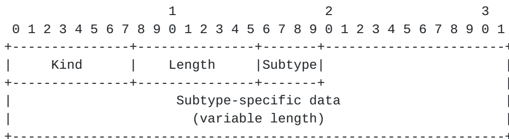
Figure 3: MPTCP Option Format
