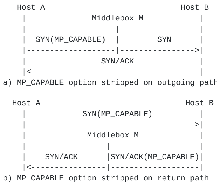
Figure 17: Connection Setup with Middleboxes that Strip Options from Packets
