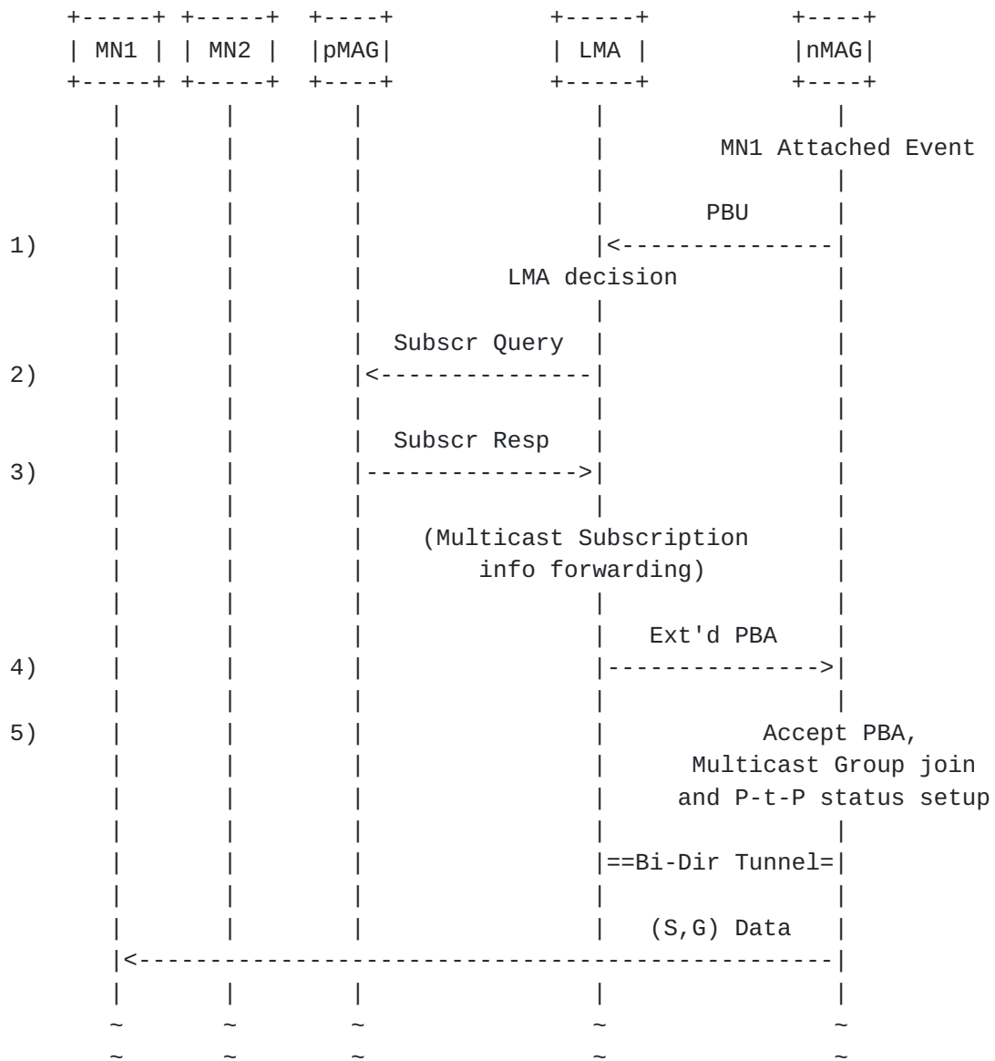
Figure 4: Reactive handover (steps 1 to 5)
