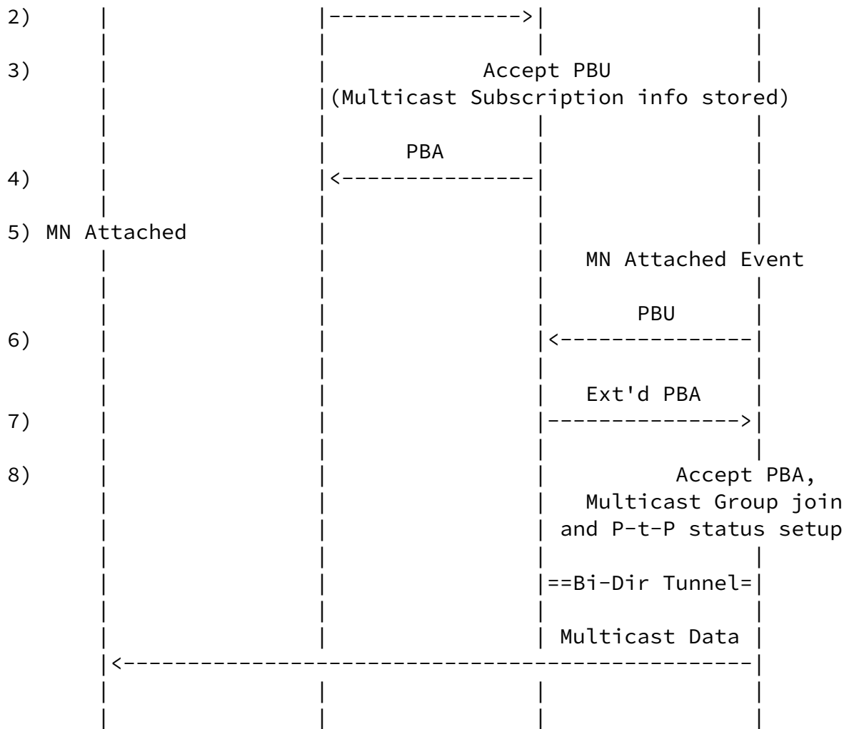
Figure 3: Proactive handover
