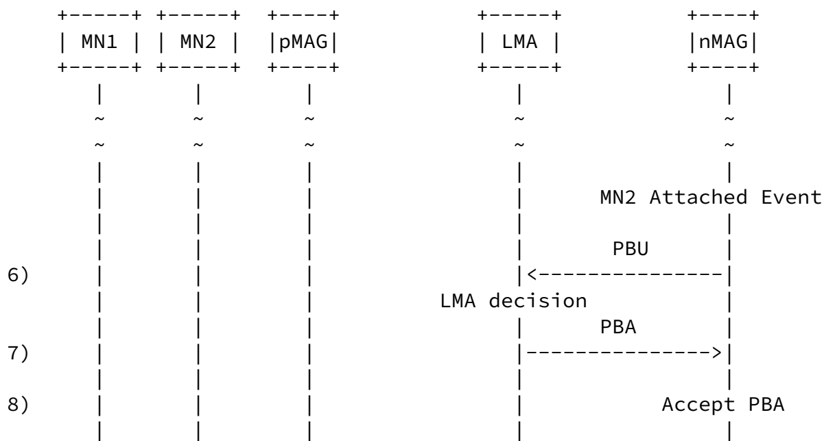
Figure 5: Reactive handover (steps 6 to 8)
