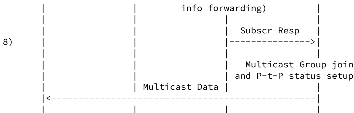
Figure 9: Decoupling of unicast and multicast signaling
