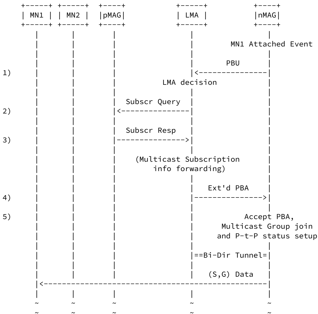
Figure 4: Reactive handover (steps 1 to 5)
