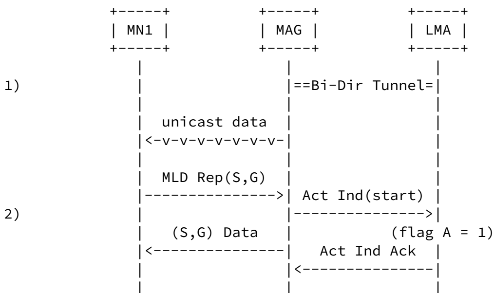
Figure 2: Multicast Activity set to ON
