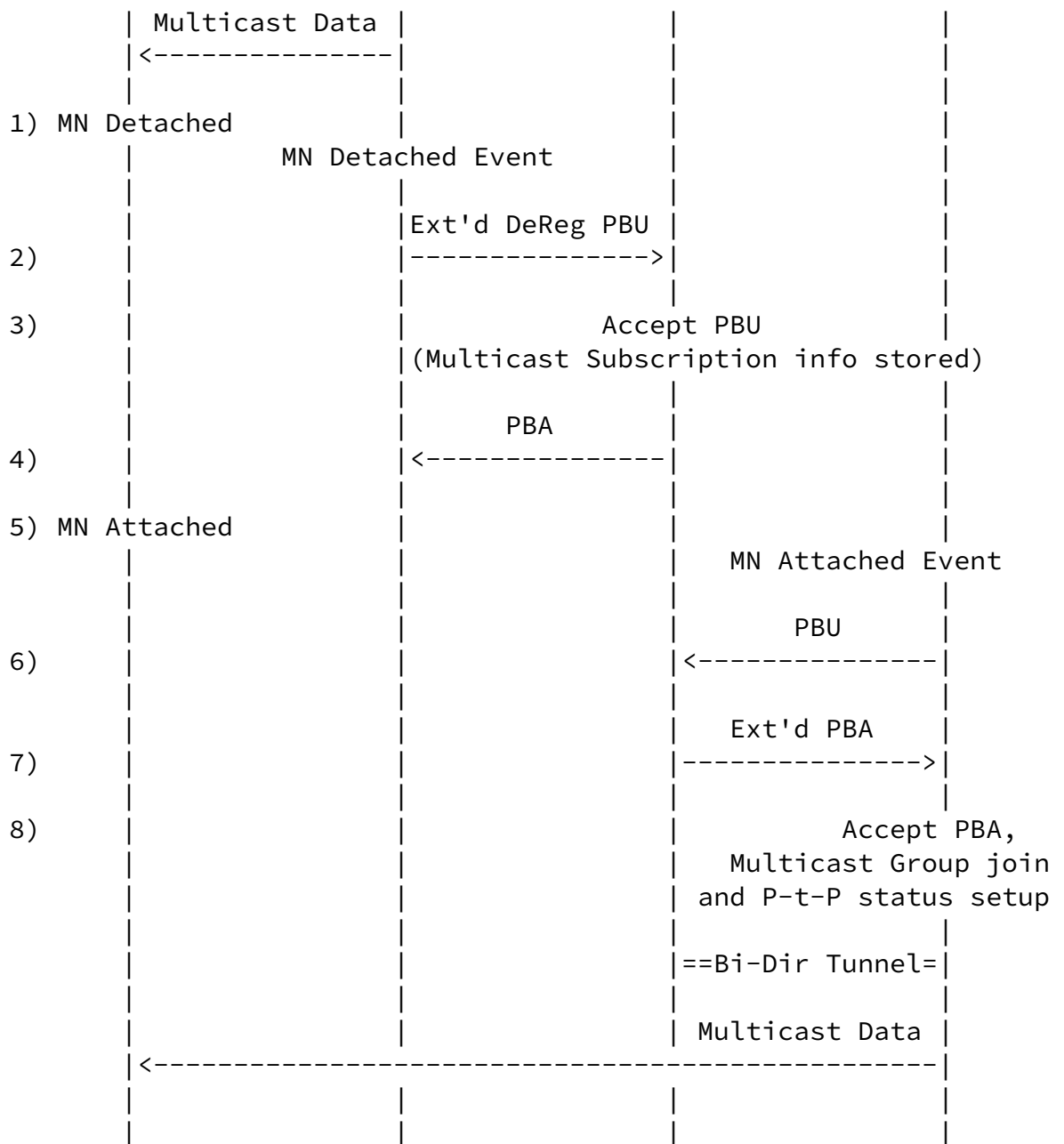
Figure 4: Proactive handover
