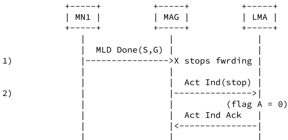
Figure 3: Multicast Activity set to OFF
