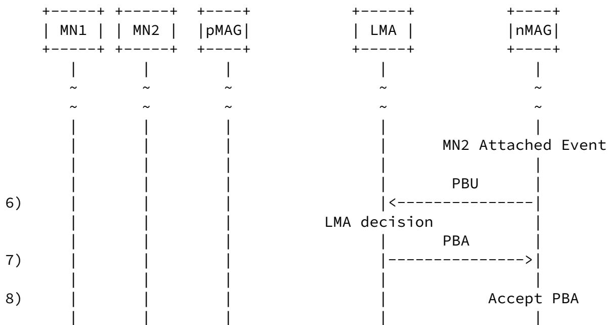
Figure 6: Reactive handover (steps 6 to 8)
