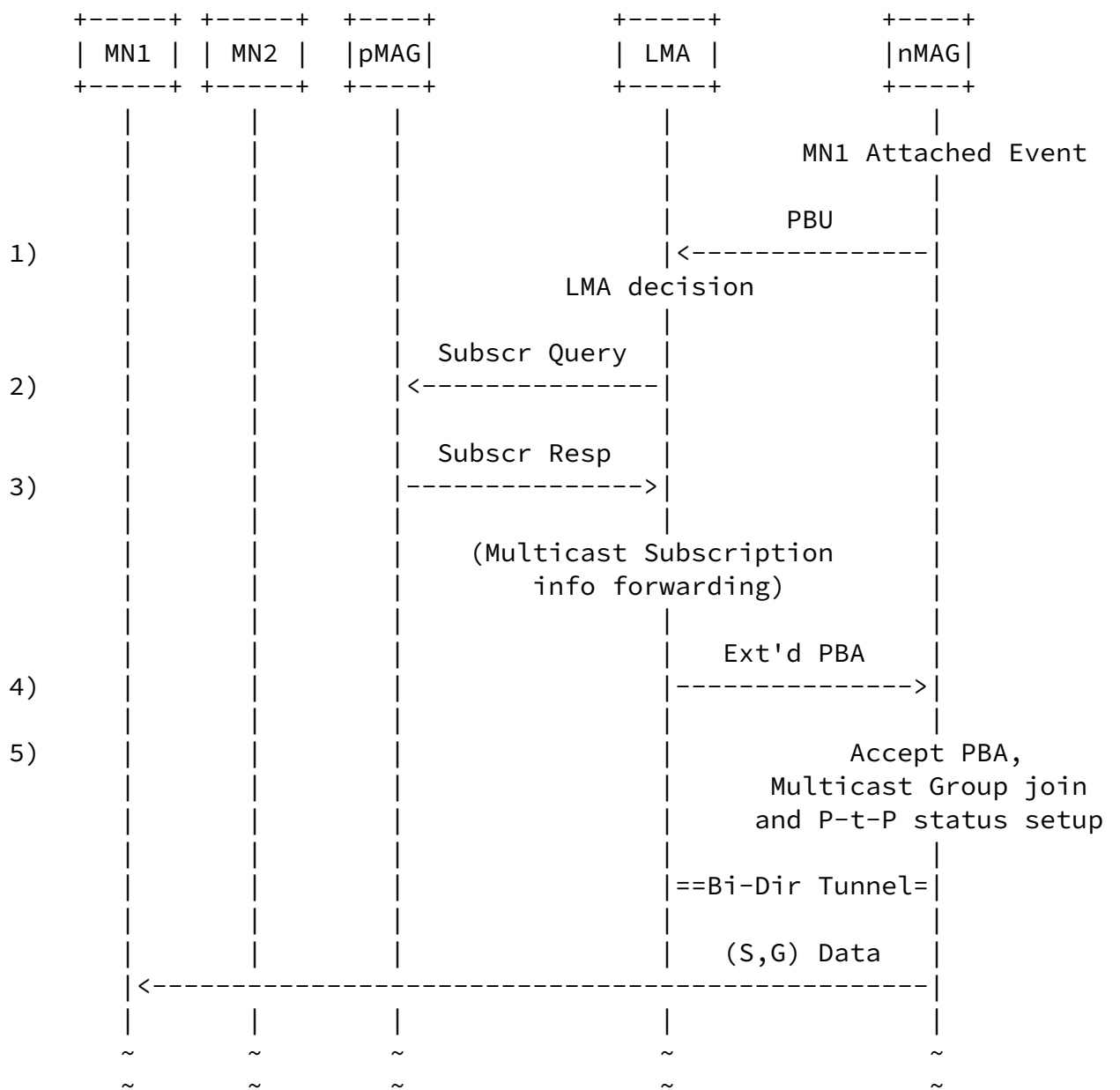
Figure 5: Reactive handover (steps 1 to 5)
