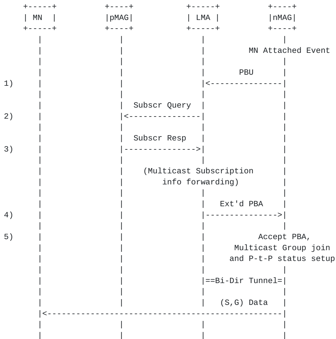
Figure 3: Reactive handover
