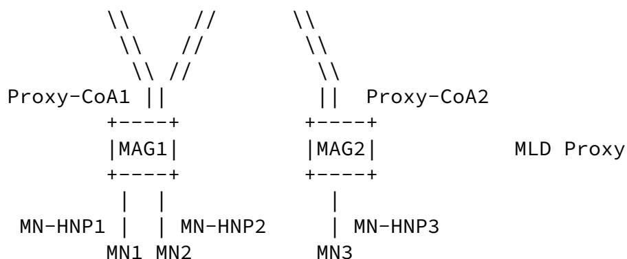
Figure 1: Reference Network for Multicast Deployment in PMIPv6
