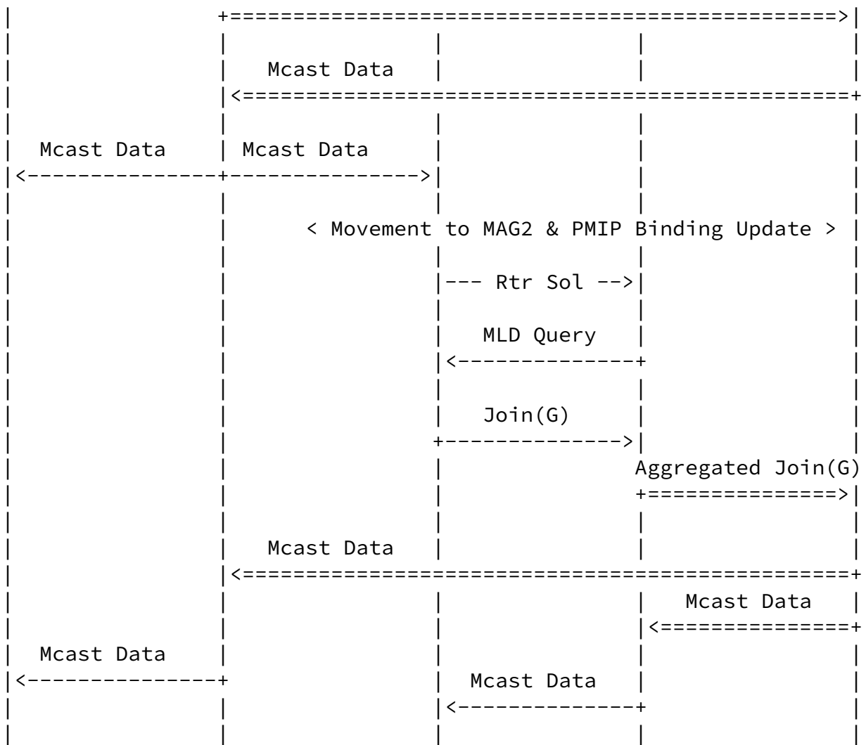
Figure 2: Call Flow of Multicast-enabled PMIP with "MLD Membership Report" abbreviated by "Join"
