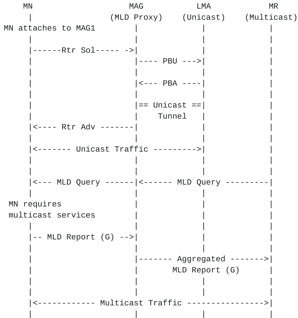
Figure 5: Multicast service establishment for direct routing
