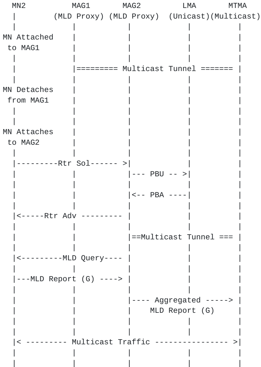
Figure 3: Multicast Mobility Signaling for MTMA
