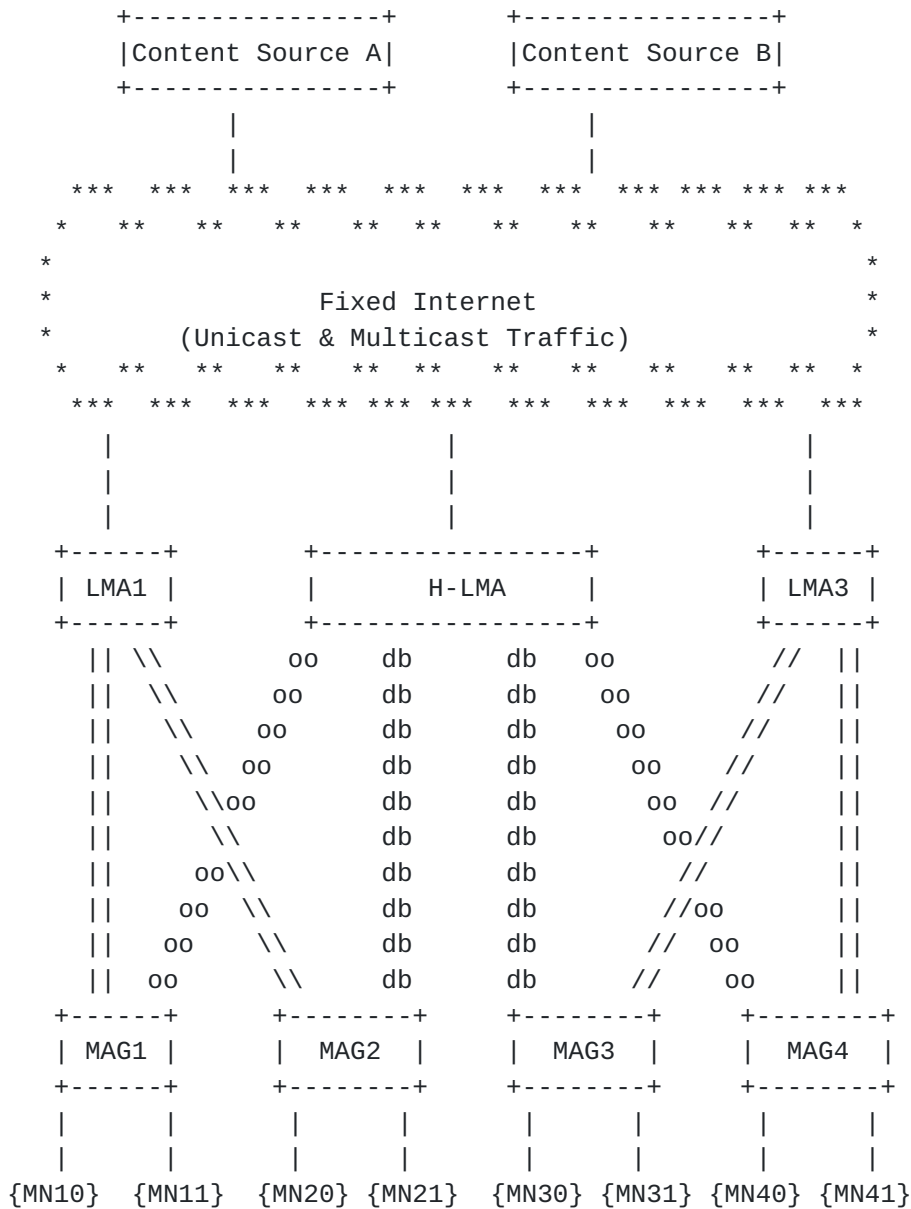
Figure 9: PMIPv6 domain with H-LMA
