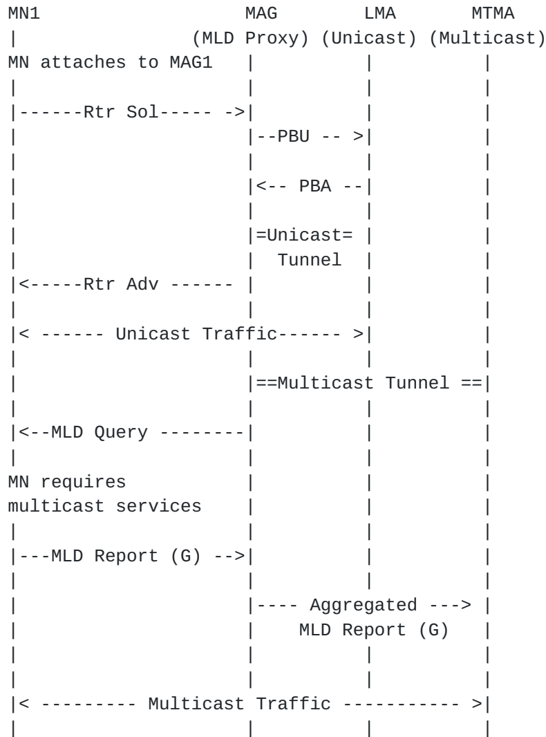
Figure 2: MN Attachment and Multicast Service Establishment for MTMA
