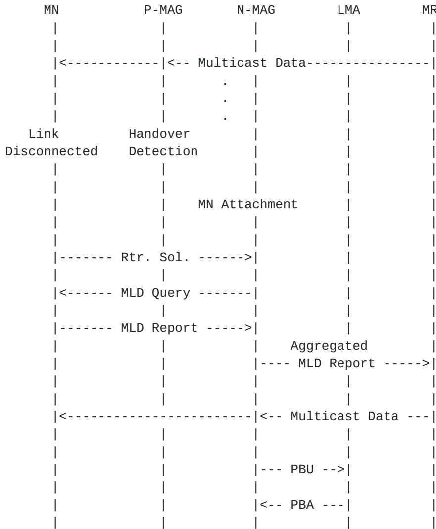
Figure 6: Multicast mobility signaling for direct routing
