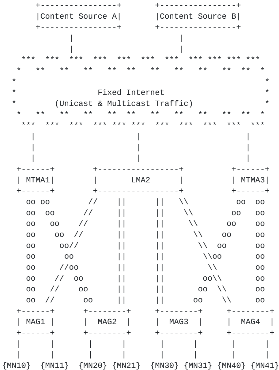
Figure 8: PMIPv6 domain with ratio 1:N
