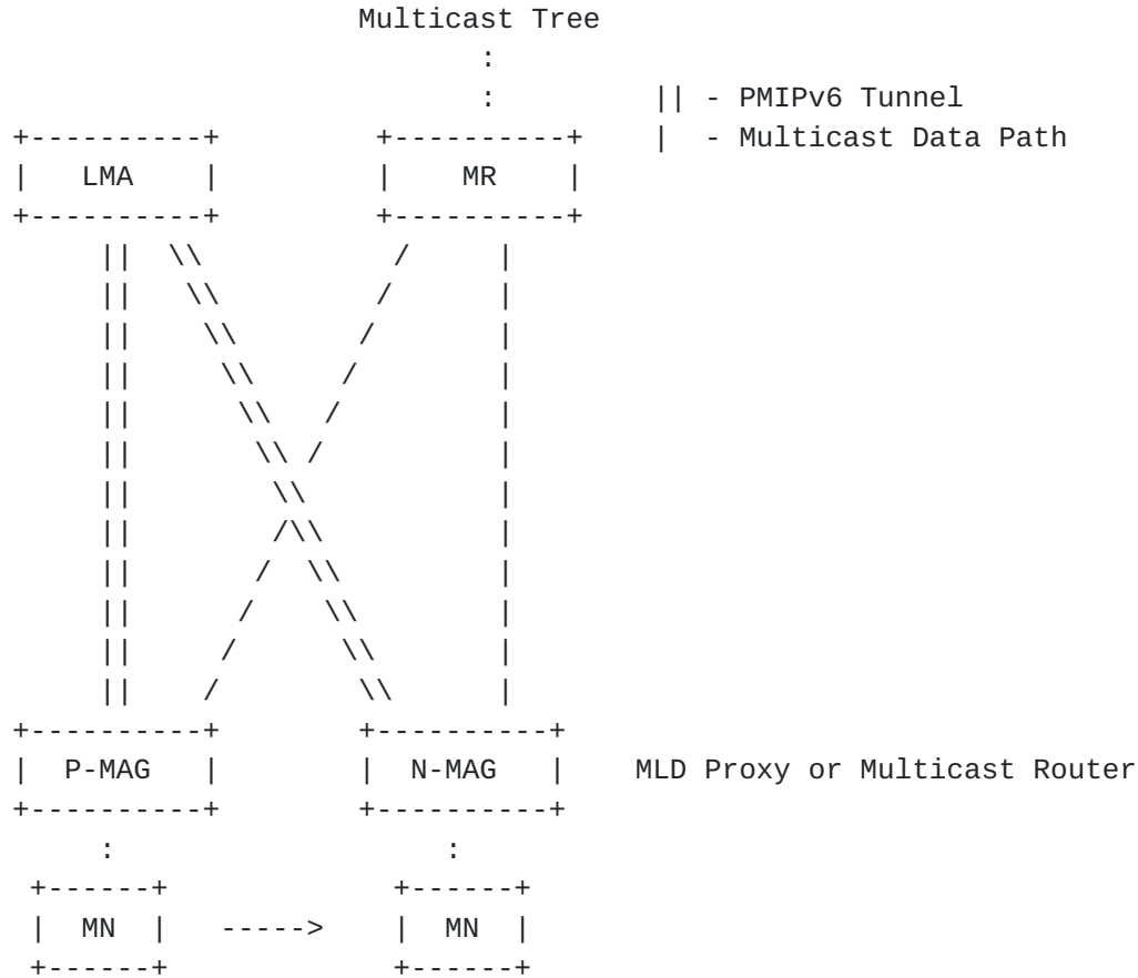
Figure 4: Architecture for direct routing based PMIPv6 multicasting
