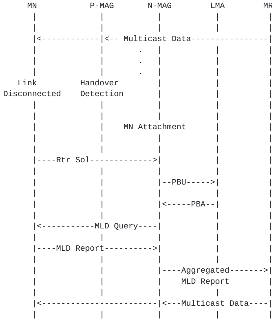
Figure 6: Multicast mobility signaling for direct routing
