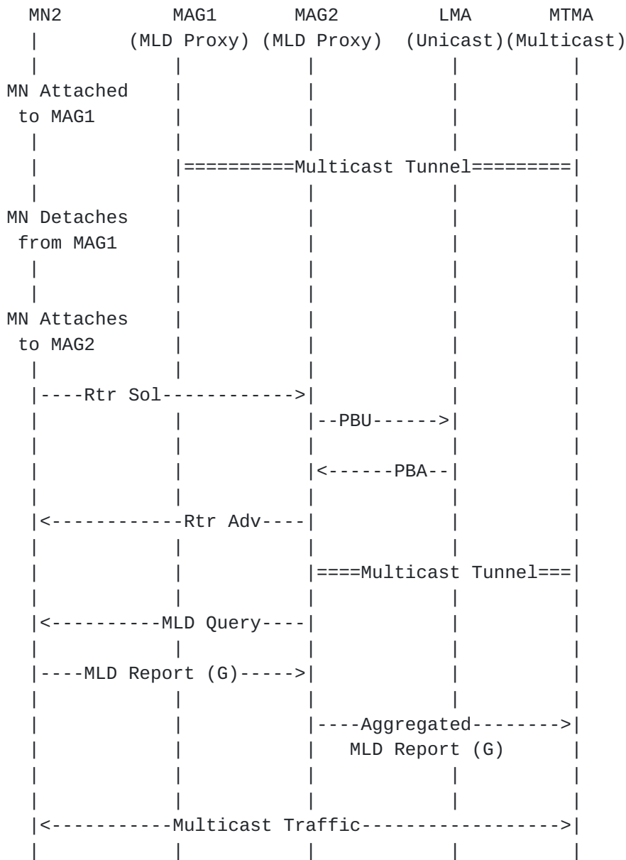
Figure 4: Multicast Mobility Signaling for MTMA
