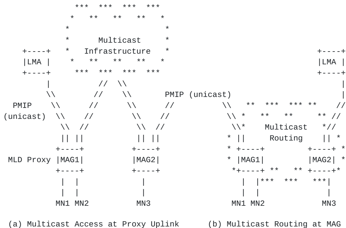
Figure 3: Reference Networks for (a) Proxy-assisted Direct Multicast Access and (b) Dynamic Multicast Routing at MAGs
