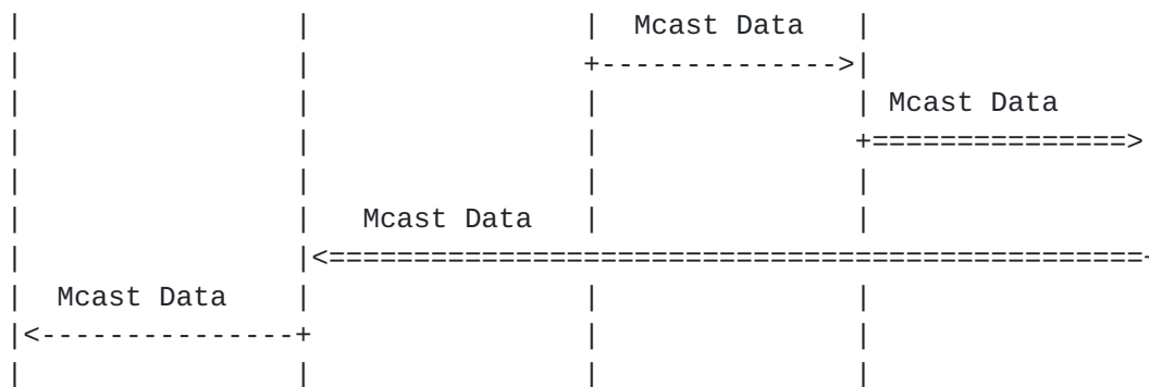
Figure 2: Call Flow for Group Communication in Multicast-enabled PMIP
