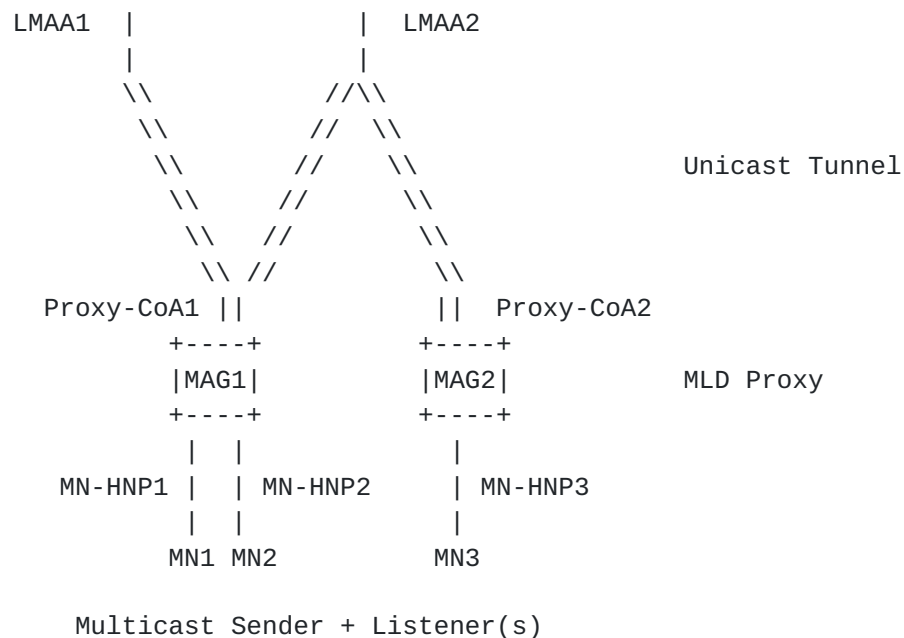
Figure 1: Reference Network for Multicast Deployment in PMIPv6 with Source Mobility - Mobile Nodes (MNs) with Home Network Prefixes (HNPs) receive services via tunnels that are spanned between a Local Mobility Anchor Address (LMAA) and a Proxy Care-of-Address (Proxy-CoA) at a Mobility Access Gateway (MAG)
