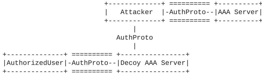
Figure 1: One Example of Original Asokan Attack
