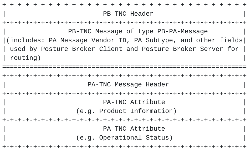
Figure 1 Overview of a PB-TNC batch that contains a PA-TNC Message
