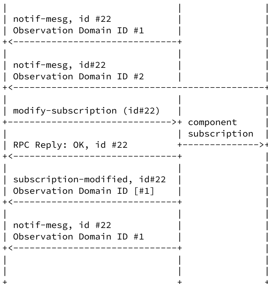
Fig. 3 Call Flow for Dynamic Subscription
