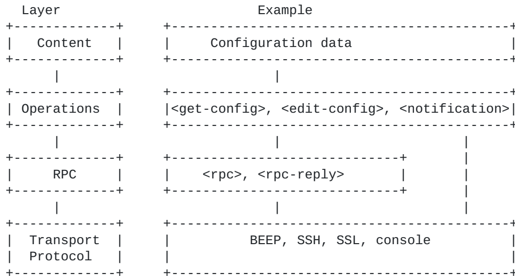
Figure 1: NETCONF layer architecture
