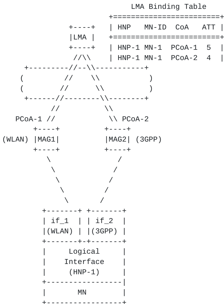
Figure 3: Multihoming Support
