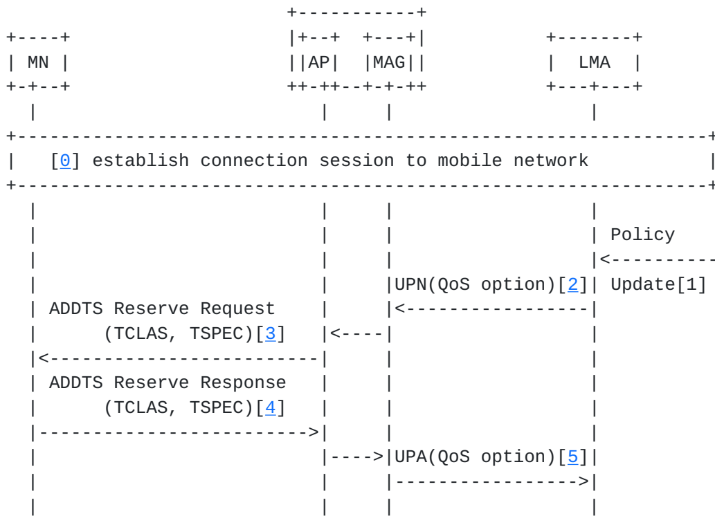
Figure 6: LMA initiated QoS service request with 802.11aa
