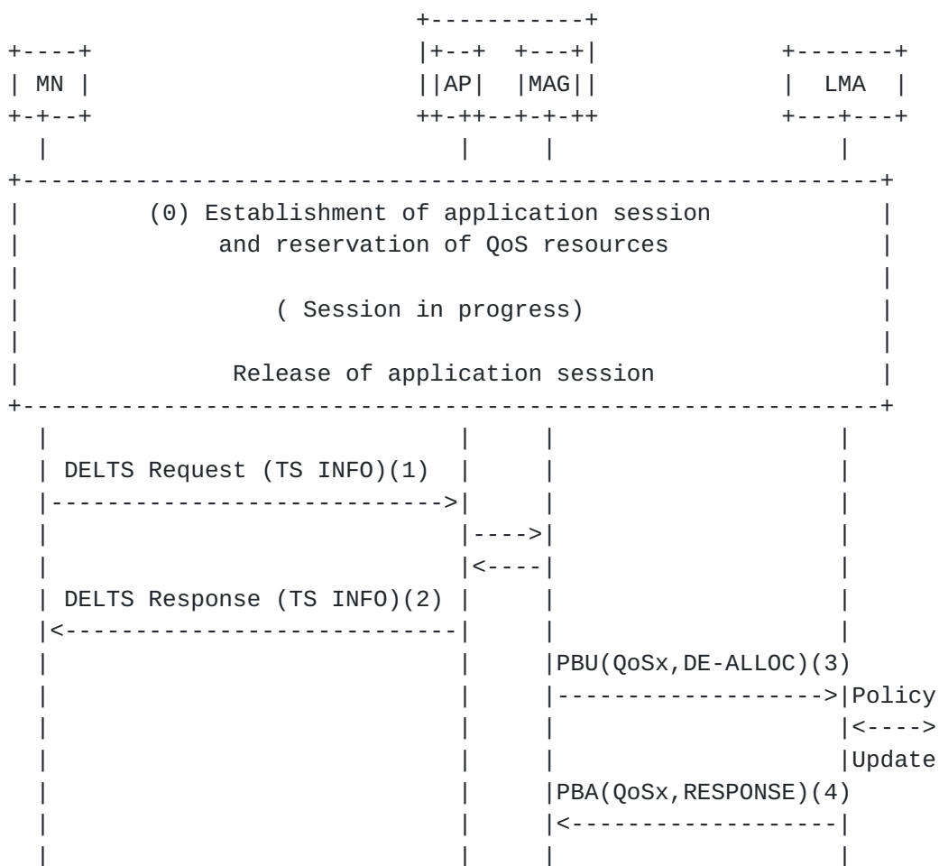
Figure 3: Network initiated QoS resource release
