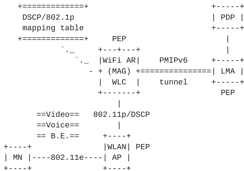
Figure 8: End-to-end QoS management with 802.11e
