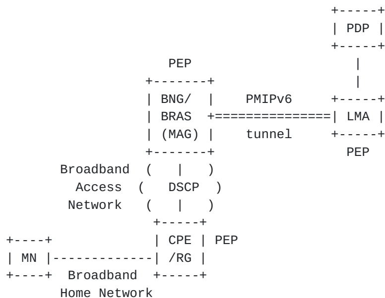
Figure 12: End-to-end QoS management with the broadband access network
