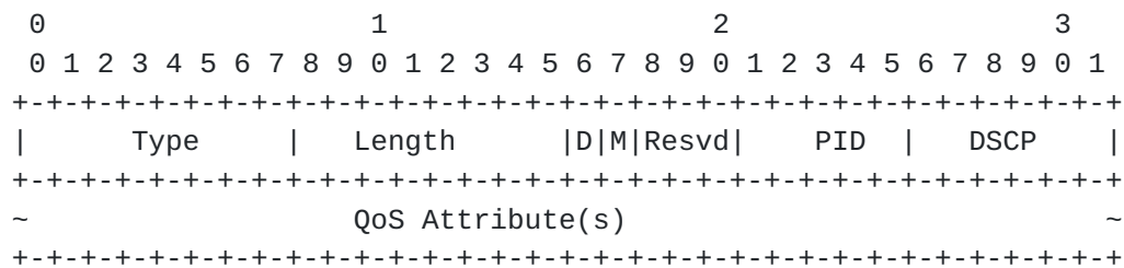
Figure 3: QoS Option
