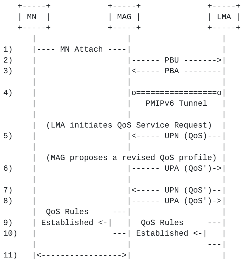
Figure 1: LMA Initiated QoS Service Request
