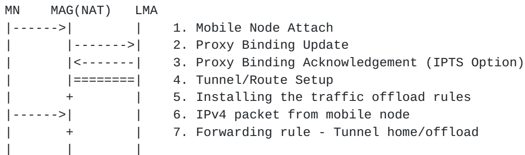
Figure 2: Exchange of IP Traffic Offload Selectors
