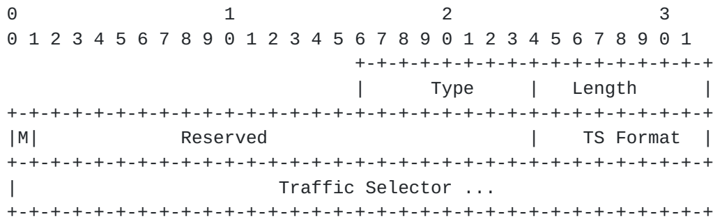
Figure 3: IP Traffic Offload Selector Option
