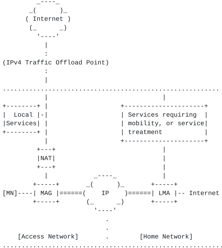
Figure 1: IP Traffic Offload Support at the MAG
