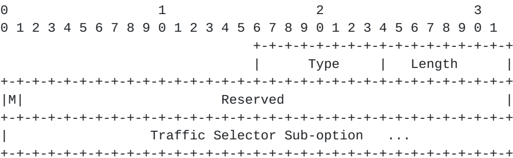
Figure 3: IPv4 Traffic Offload Selector Option
