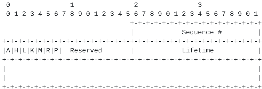
Figure 11: Proxy Binding Update Message
