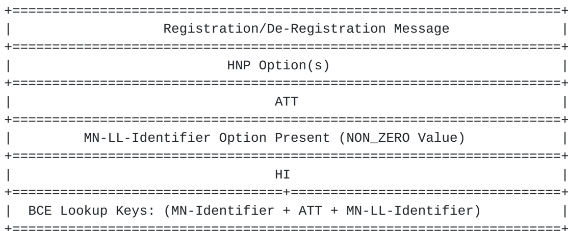
Figure 7: BCE Lookup using Link-layer Identifier
