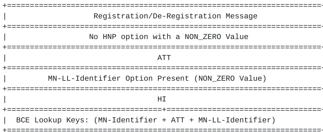
Figure 8: BCE Lookup using Link-layer Identifier
