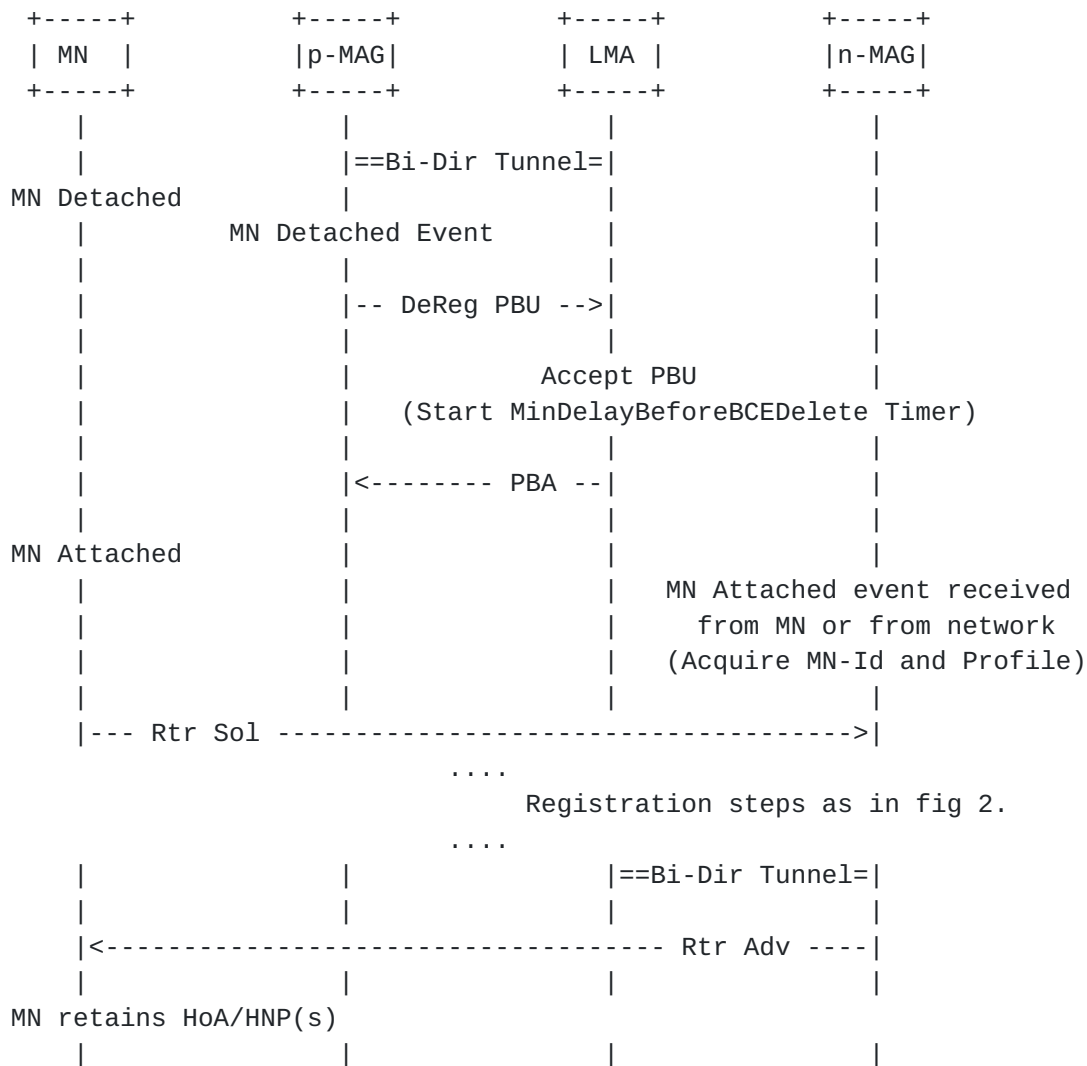
Figure 3: Mobile Node Handoff - Signaling Call Flow
