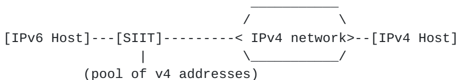
Figure 1. Using SIIT for a single IPv6-only subnet.
