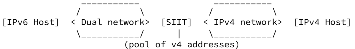
Figure 2. Using SIIT for an IPv6-only or dual cloud (e.g. a site) which contains some IPv6-only hosts as well as IPv4 hosts.
