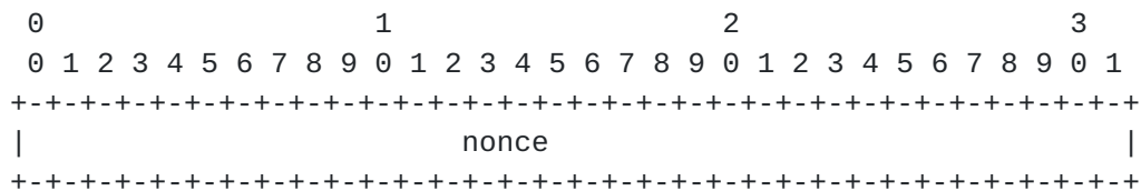
Figure 26: Nonce Object
