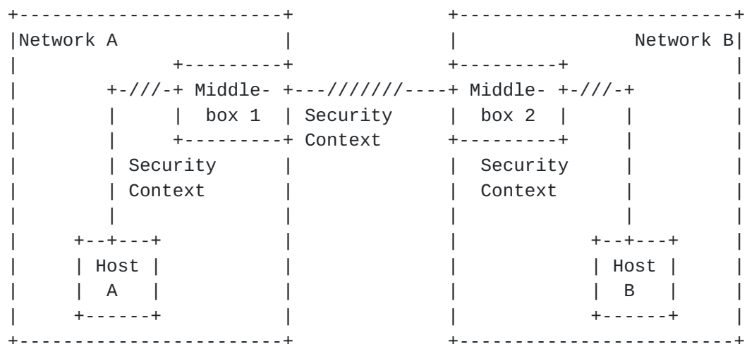
Figure 30: Peer-to-Peer Relationship
