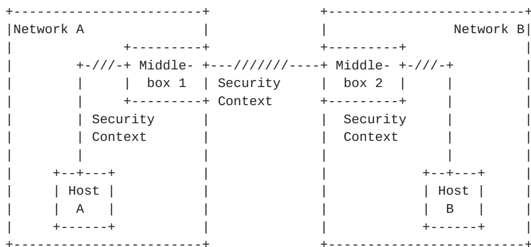
Figure 31: Peer-to-Peer Relationship
