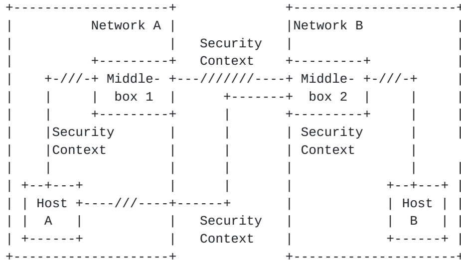
Figure 33: End-to-Middle Relationship
