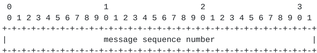
Figure 28: Message Sequence Number Object
