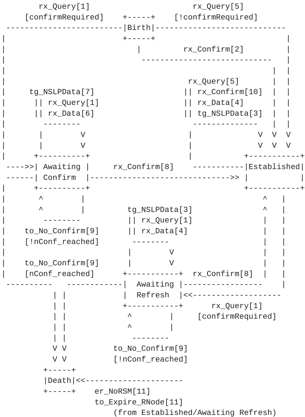
Figure 8: Responder Node State Machine
