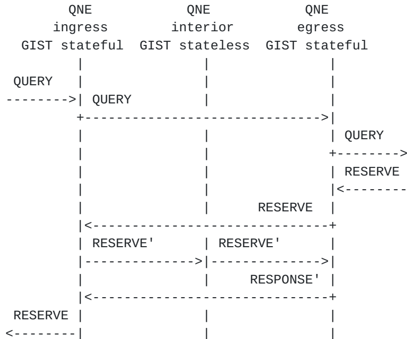
Figure 15: Receiver-initiated reservation with Reduced State Interior Nodes
