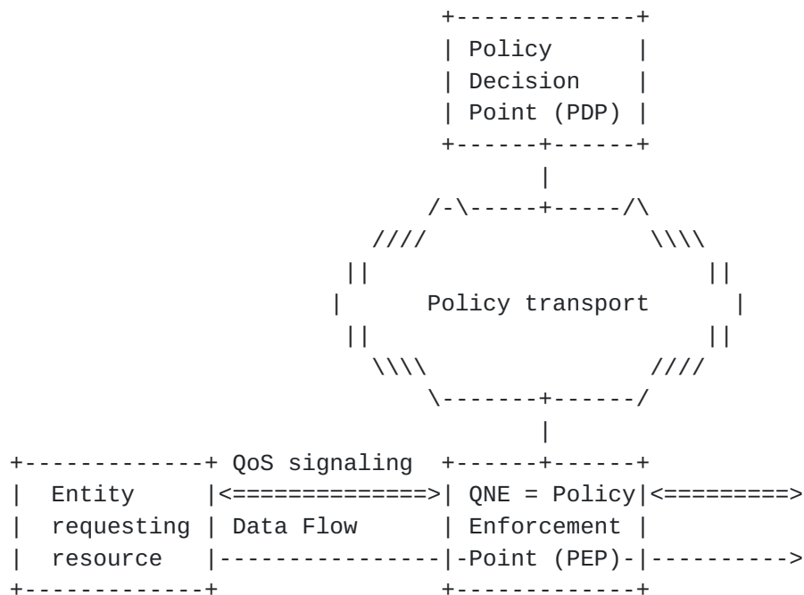
Figure 3: Policy control with the QoS NSLP signaling
