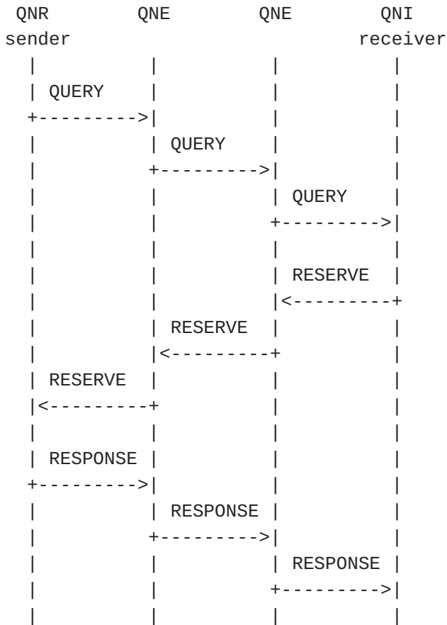
Figure 8: Basic Receiver Initiated Reservation
