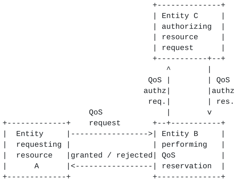
Figure 19: Three party approach
