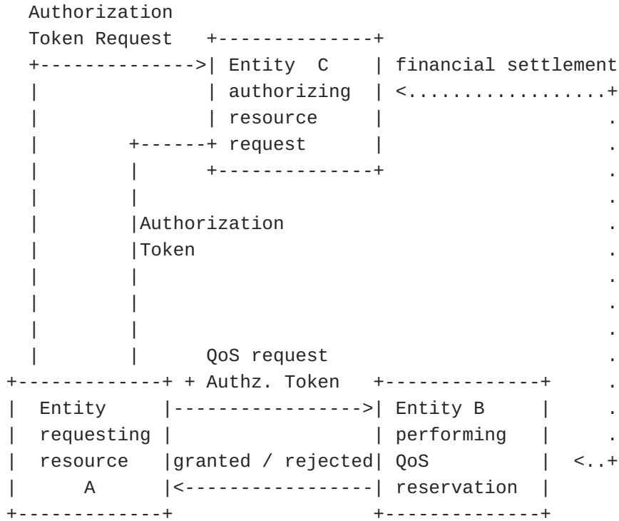
Figure 18: Token based three party approach
