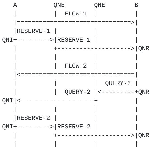
Figure 10: Bi-directional reservation for sender+receiver scenario
