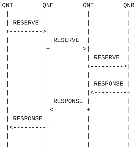
Figure 7: Basic Sender Initiated Reservation
