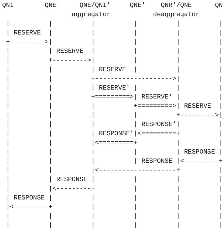
Figure 11: Sender Initiated Reservation with Aggregation
