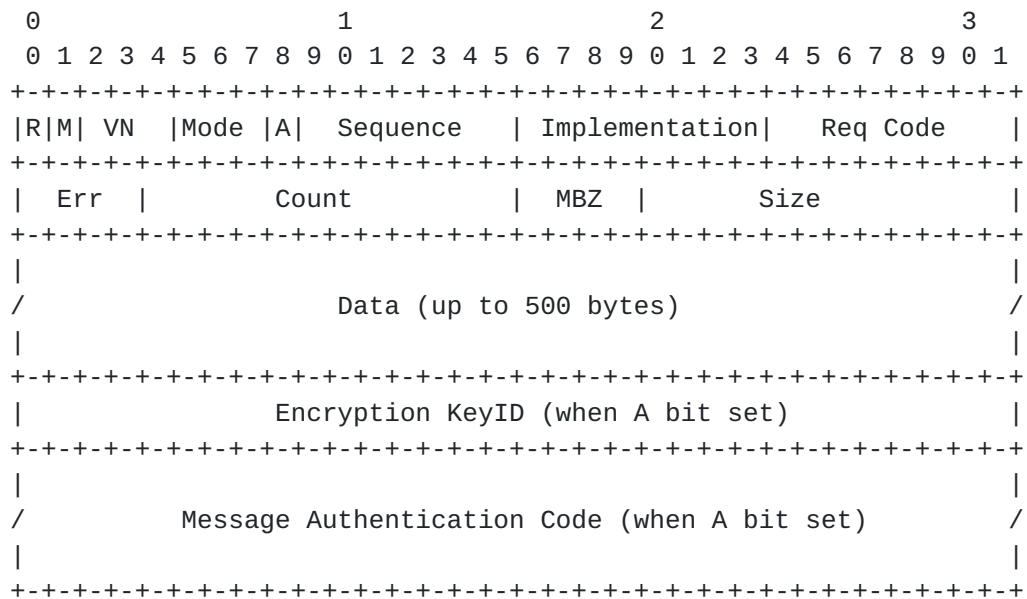
Figure 3: NTP Remote Facility Message Header
