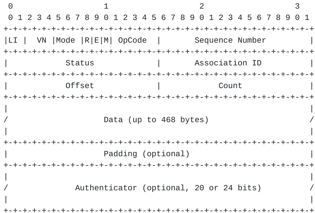
Figure 1: NTP Control Message Header
