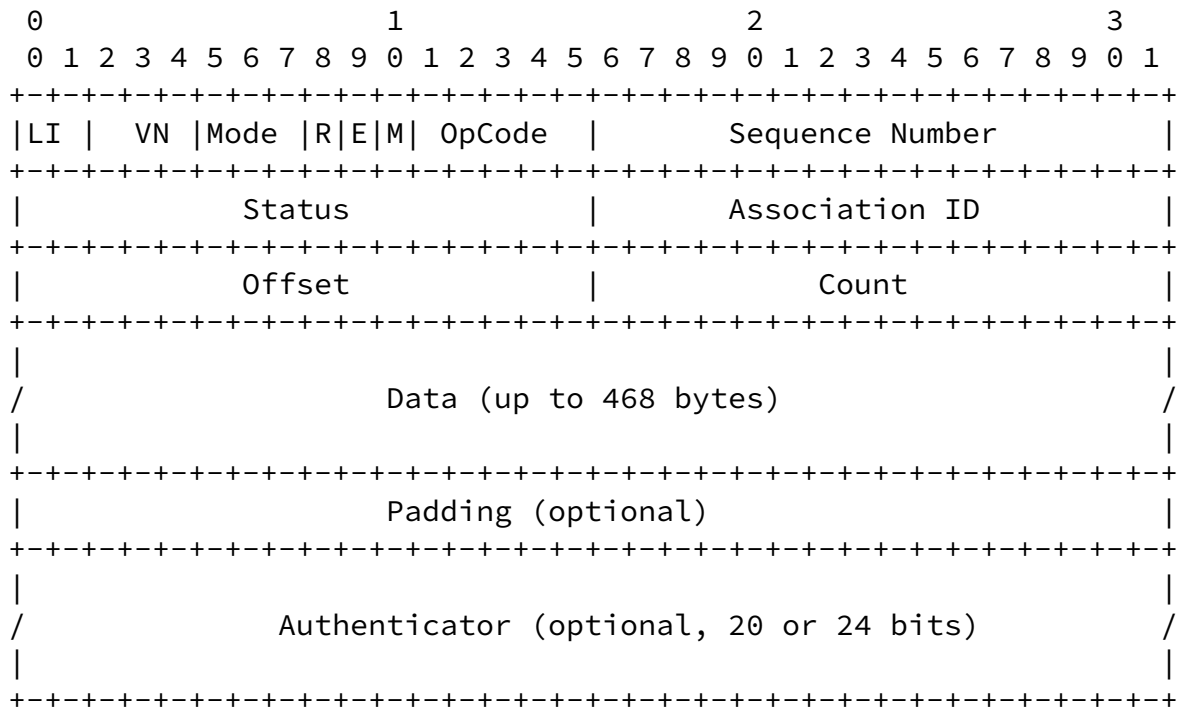
Figure 1: NTP Control Message Header
