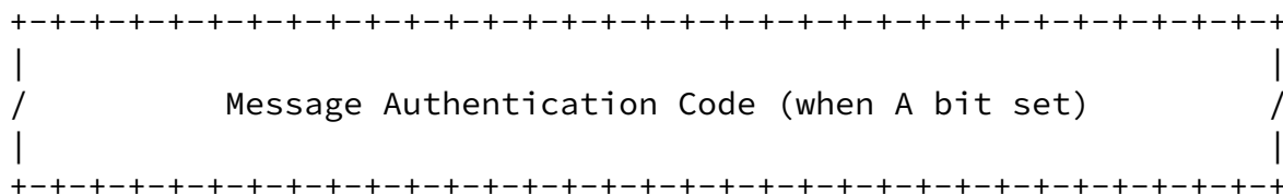
Figure 3: NTP Remote Facility Message Header
