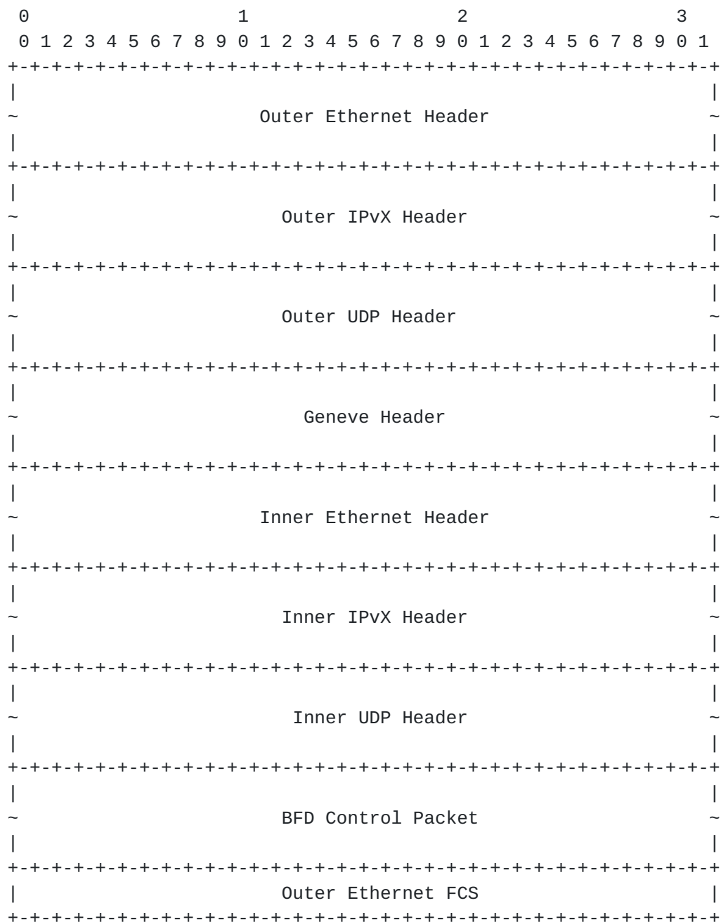
Figure 1: Geneve Encapsulation of BFD Control Packet With the Inner Ethernet/IP/UDP Header
