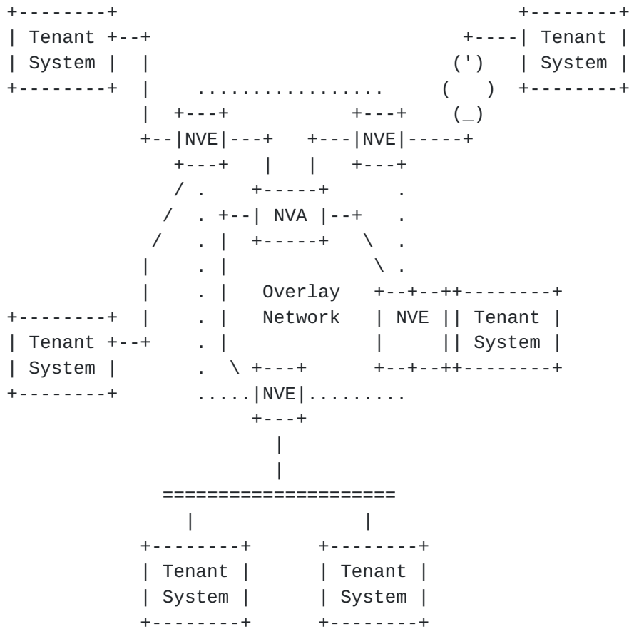
Figure 2 : Generic reference model for DC network virtualization overlay
