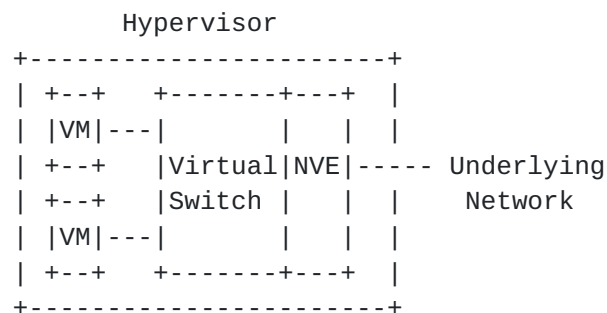
Hypervisor with an Embedded NVE.
