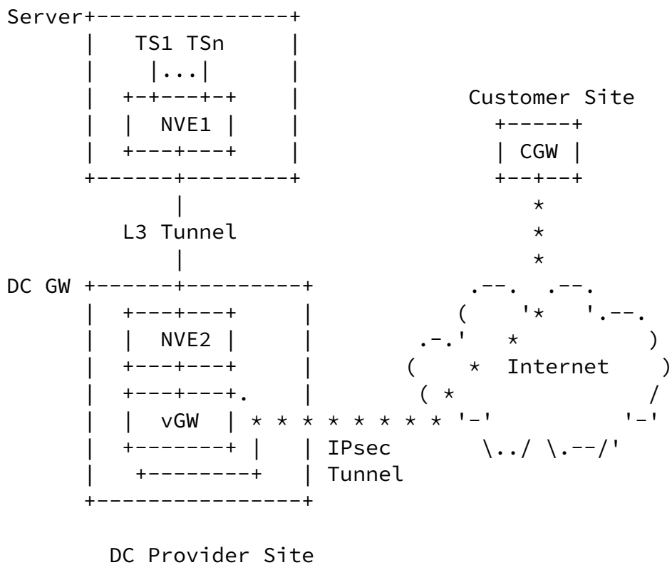
Figure 1 - DC Virtual Network Access via the Internet
