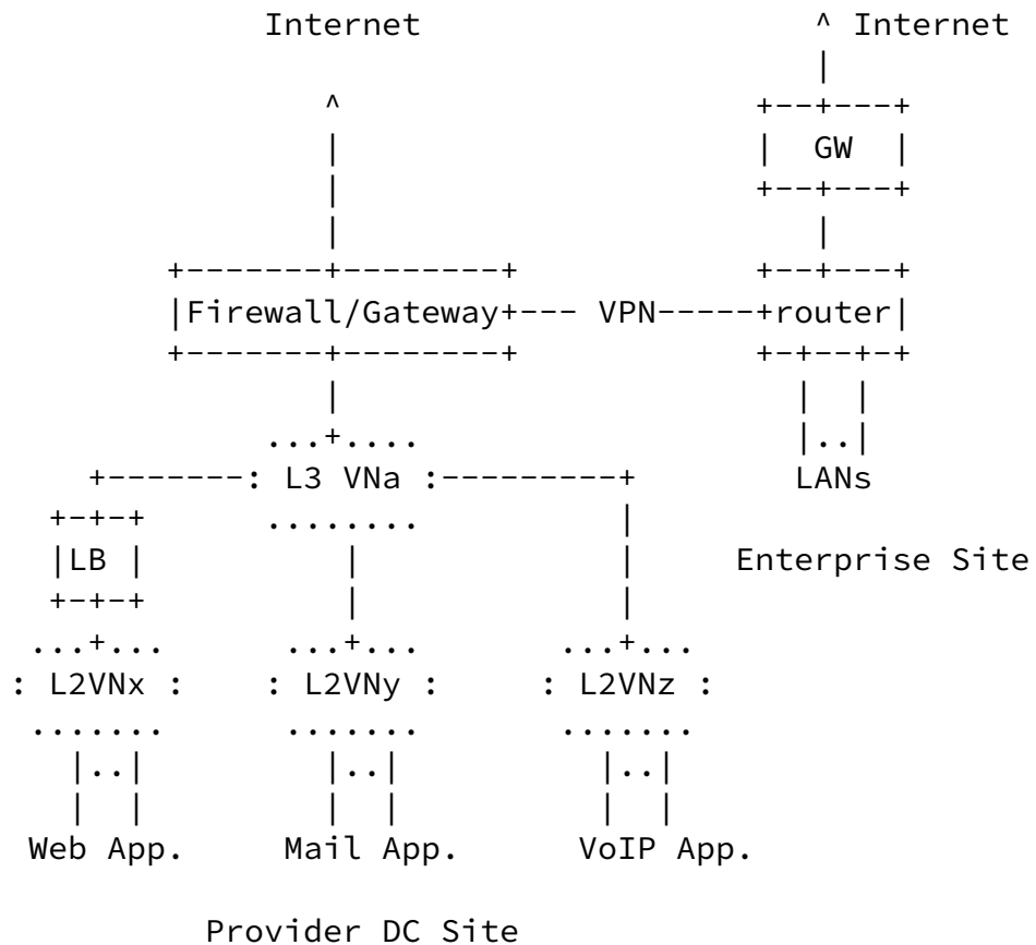
Figure 2 - Virtual Data Center Abstraction View
