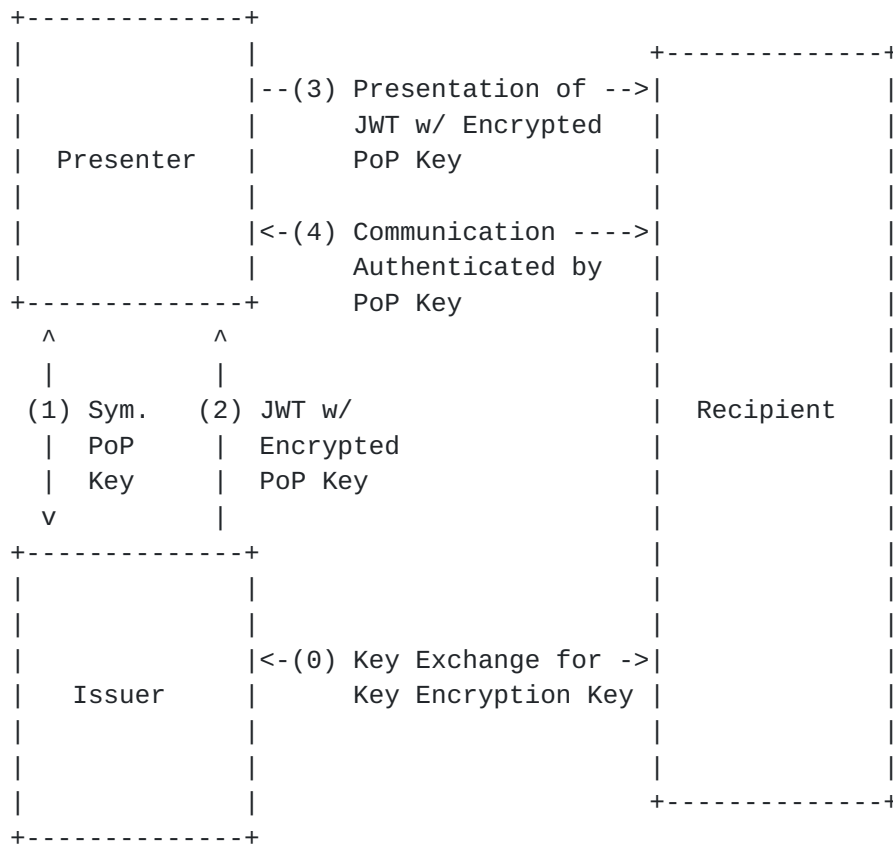
Figure 1: Proof-of-Possession with a Symmetric Key
