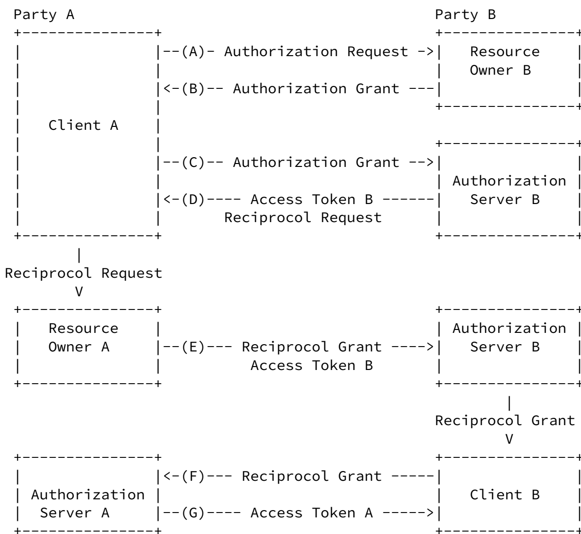
Figure 1: Abstract Reciprocal Protocol Flow
