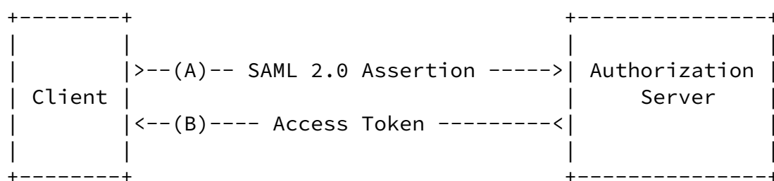
Figure 1: Assertion Access Token Request
