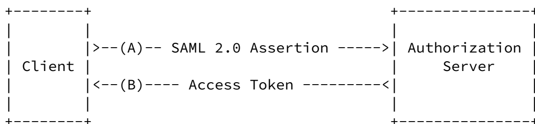
Figure 1: Assertion Access Token Request
