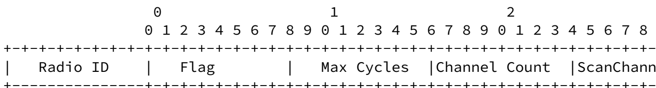
Figure 6: IEEE 802.11 Scan Channel Bind Message Element
