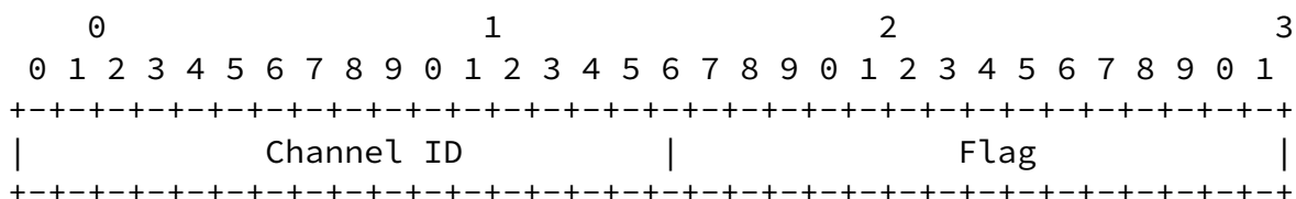
Figure 7: Channel Information Format
