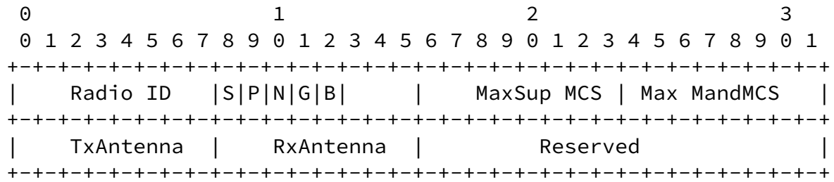
Figure 1: 802.11n Radio Configuration Message Element
