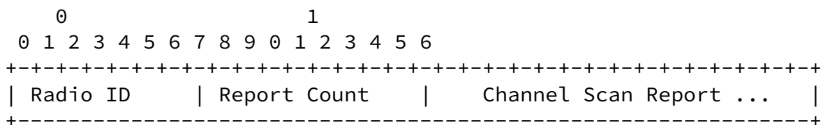
Figure 8: IEEE 802.11 Channel Scan Report Message Element
