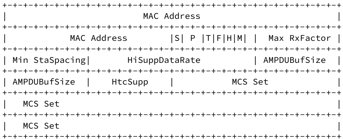
Figure 3: 802.11n Station Information
