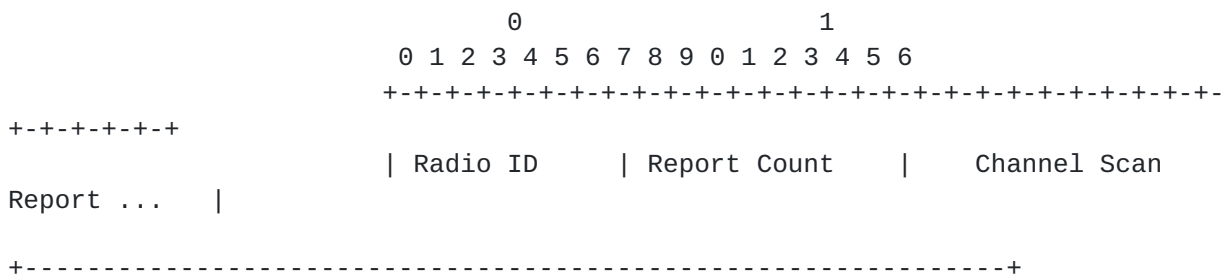
Figure 8: IEEE 802.11 Channel Scan Report Message Element
