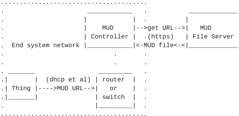
Figure 1: MUD Architecture
