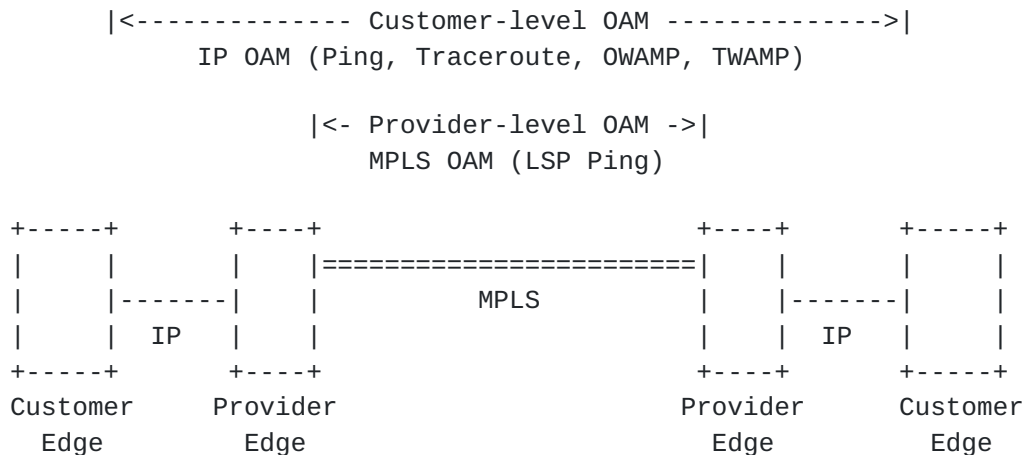
Figure 1 Example: Multi-layer OAM
